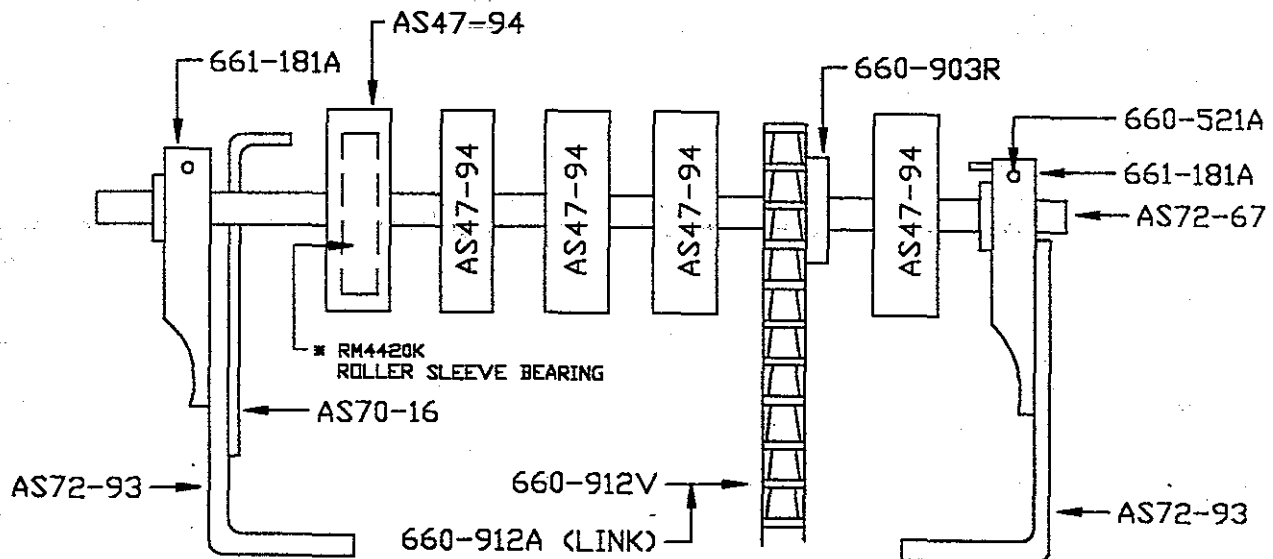
TAILSHAFT-RIGHT LOADING
